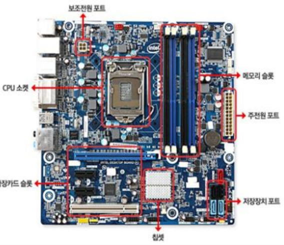
Embedded Board
